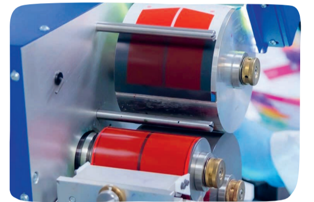
Fixed Anilox Printing.
