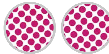
Dot reproduction: 4000dpi VS 9600dpi
